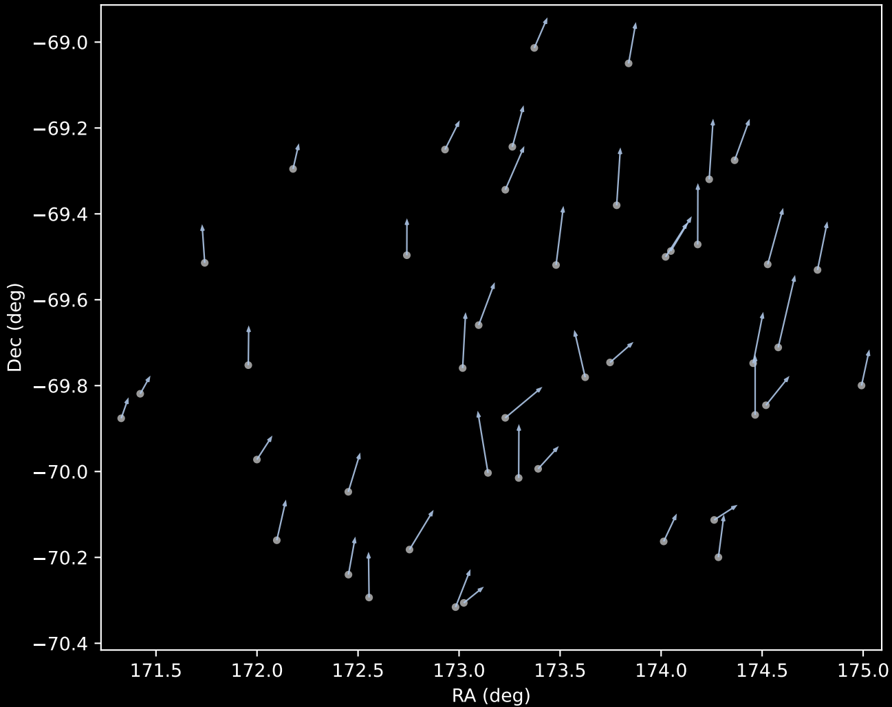
GALAH DR4 Cluster 1 Proper Motion Vectors (n=44)
