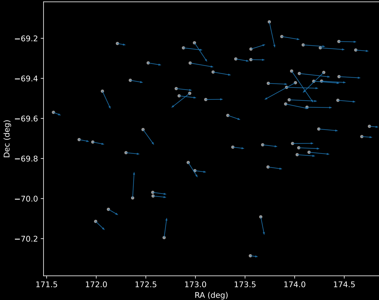
GALAH DR4 Cluster 0 Proper Motion Vectors (n=60)
