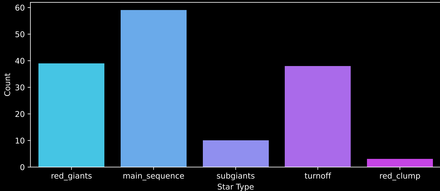
GALAH DR4 Field: [467] Count plot of Star Type
