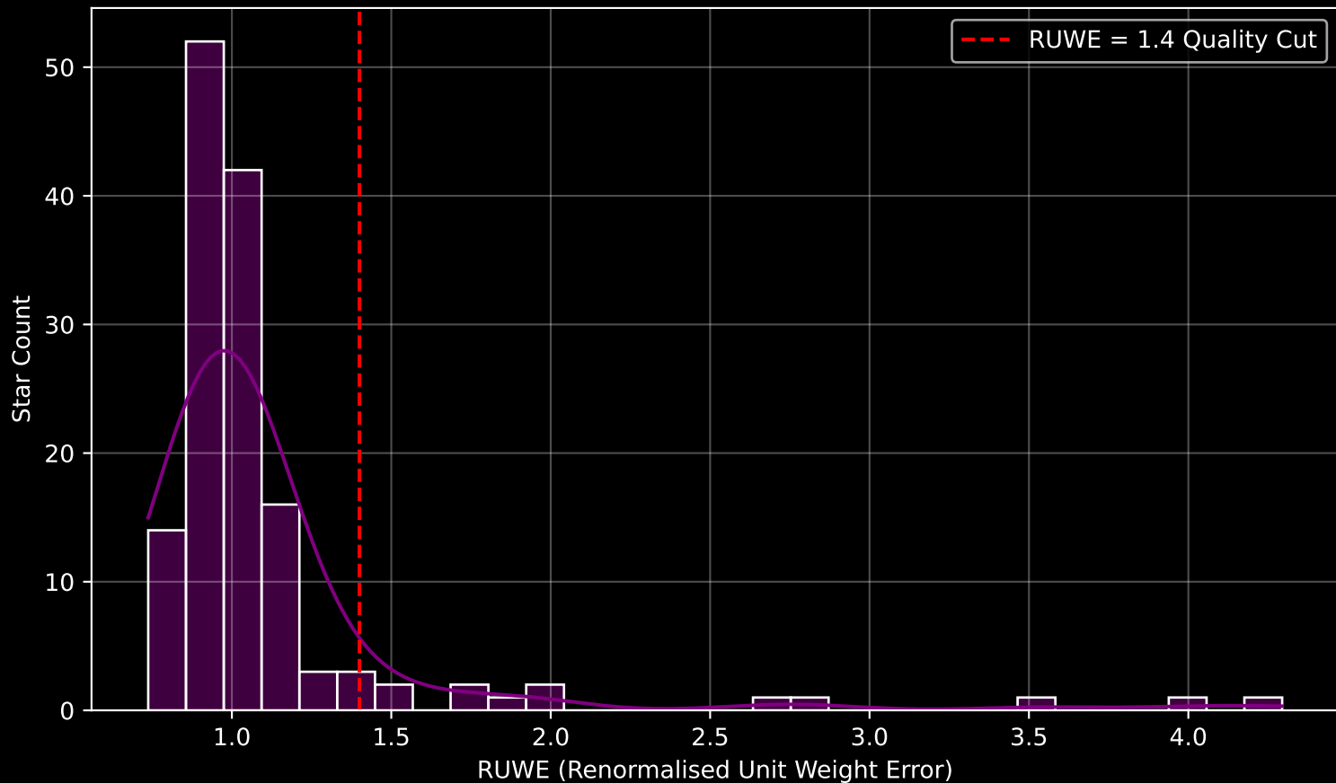
GALAH DR4 Field [467] RUWE Distribution (n= 142)
